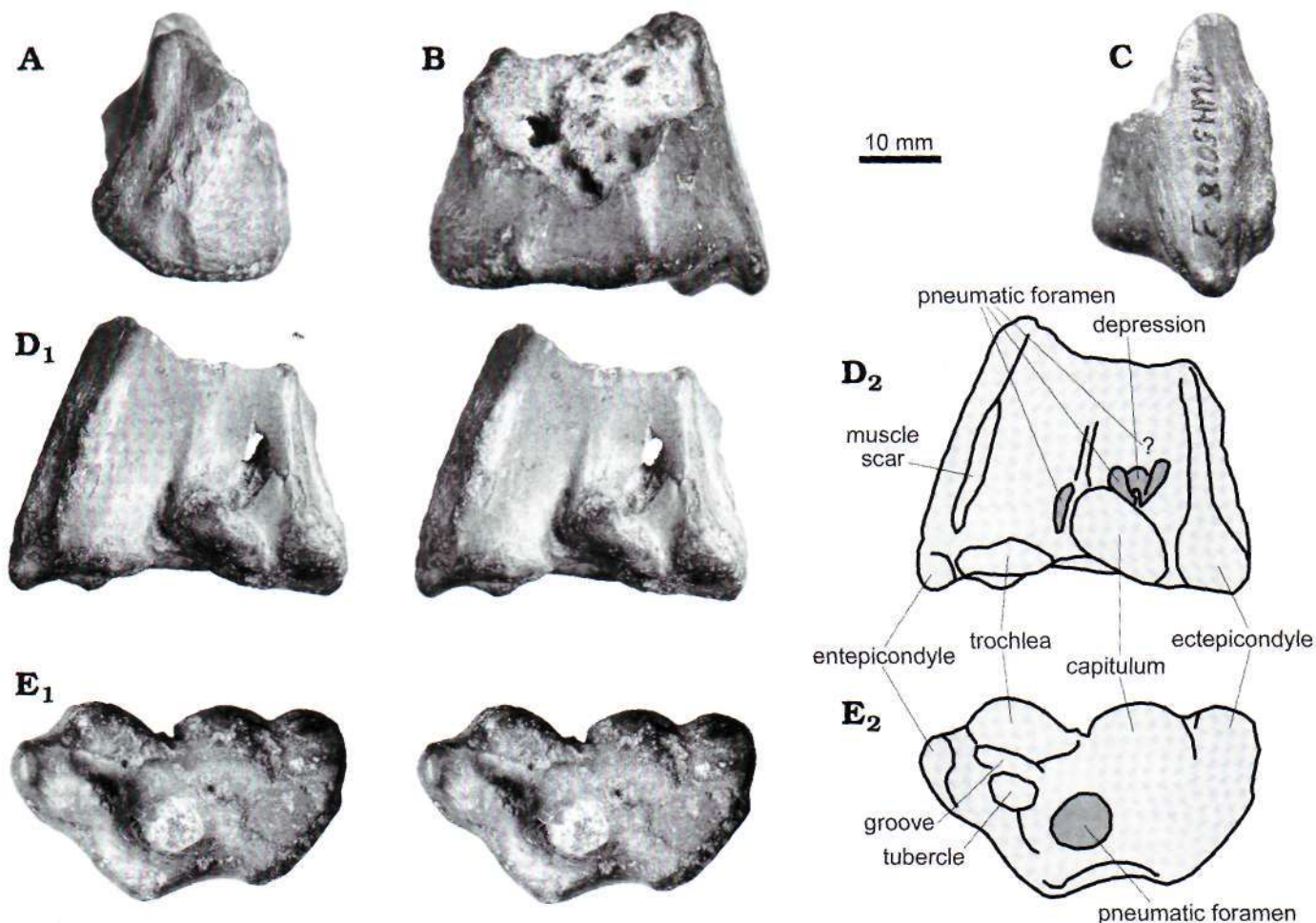
Fig. 2. Ormithocheiroidea indet. PIN 5028-3, left humerus distal end. Melovatka 3, Volgograd Region, Russia; Upper Cretaceous, upper Cenomanian; in anterior (A), dorsal (B), posterior (C), ventral (D), and distal (E) views. D 1 and E 1 are stereo-photographs with explanatory drawings (D 2 , E 2 ). The oval opening seen in right upper corner of the stereo-photograph in Fig. D 1 is a postmortem bone breakage and therefore it is not shown in explanatory drawing.
