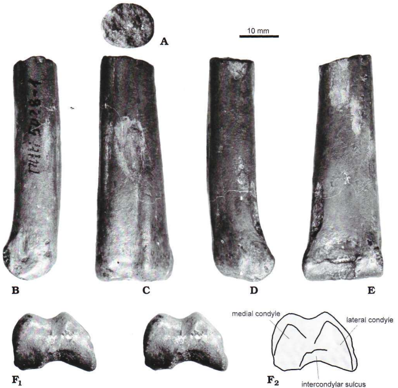
Fig. 3. Ornithocheiroidea indet. PIN 5028-1, left femur distal end. Melovatka 3, Volgograd Region, Russia; Upper Cretaceous, upper Cenomanian. Cross-section of the diaphysis (A), medial view (B), anterior view (C), lateral view (D), posterior view (E), and distal view (F). F 1 is a stereo-photograph with explanatory drawing (F 2 ).
